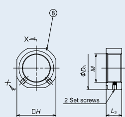
Lock nut
