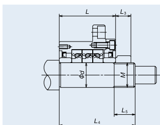
Dimension of bearing seat
