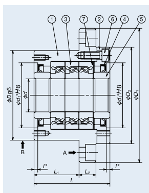
Components of support unit
