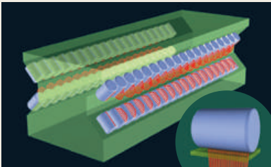
Analysis example of contact pressure distribution of rollers
