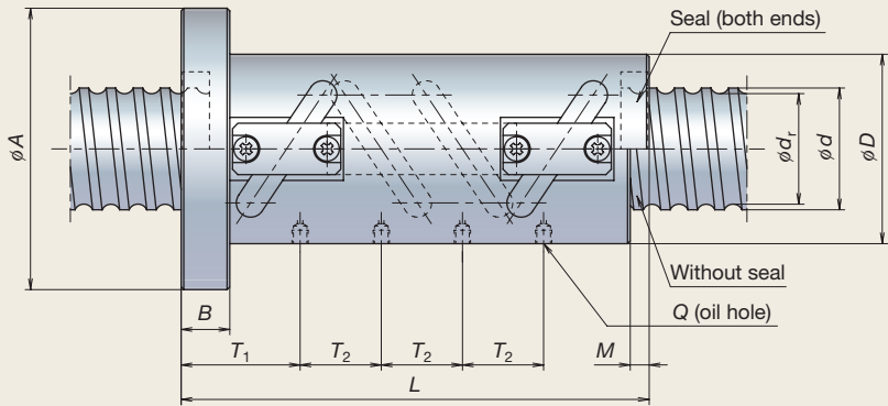
Nut model III
