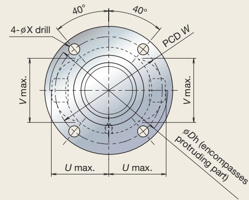
Outline drawing
