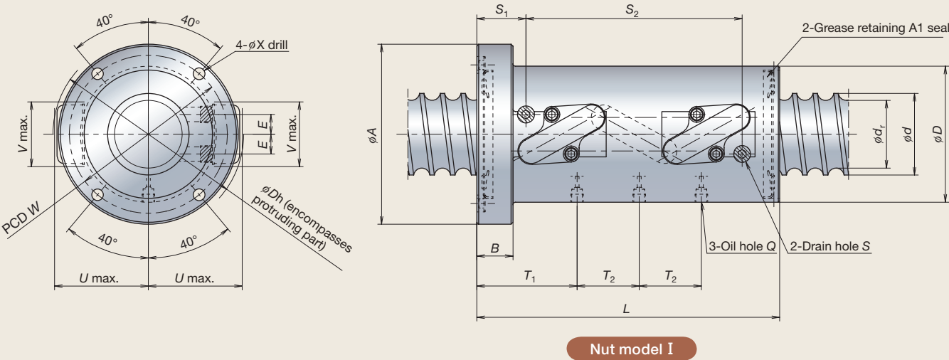
Outline drawing
