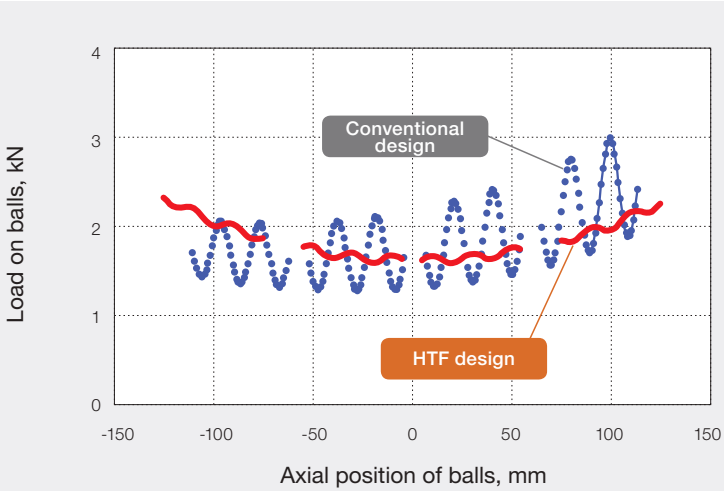
Load distribution to balls
